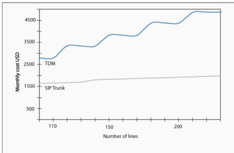
Figure 5 -Cost to expand infrastructure. TDM vs. SIP trunks.
