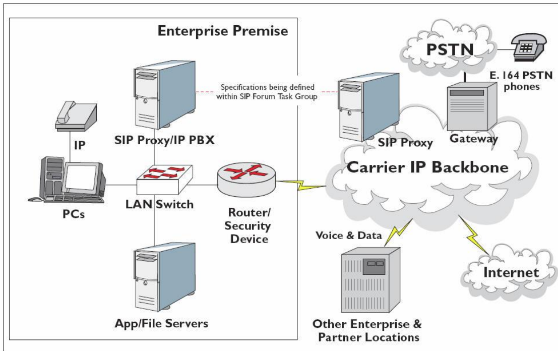
Figure 1 Typical SIP trunking solution
